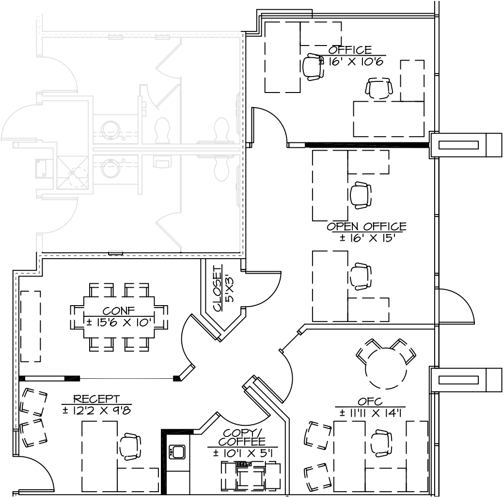
FLOOR PLAN
